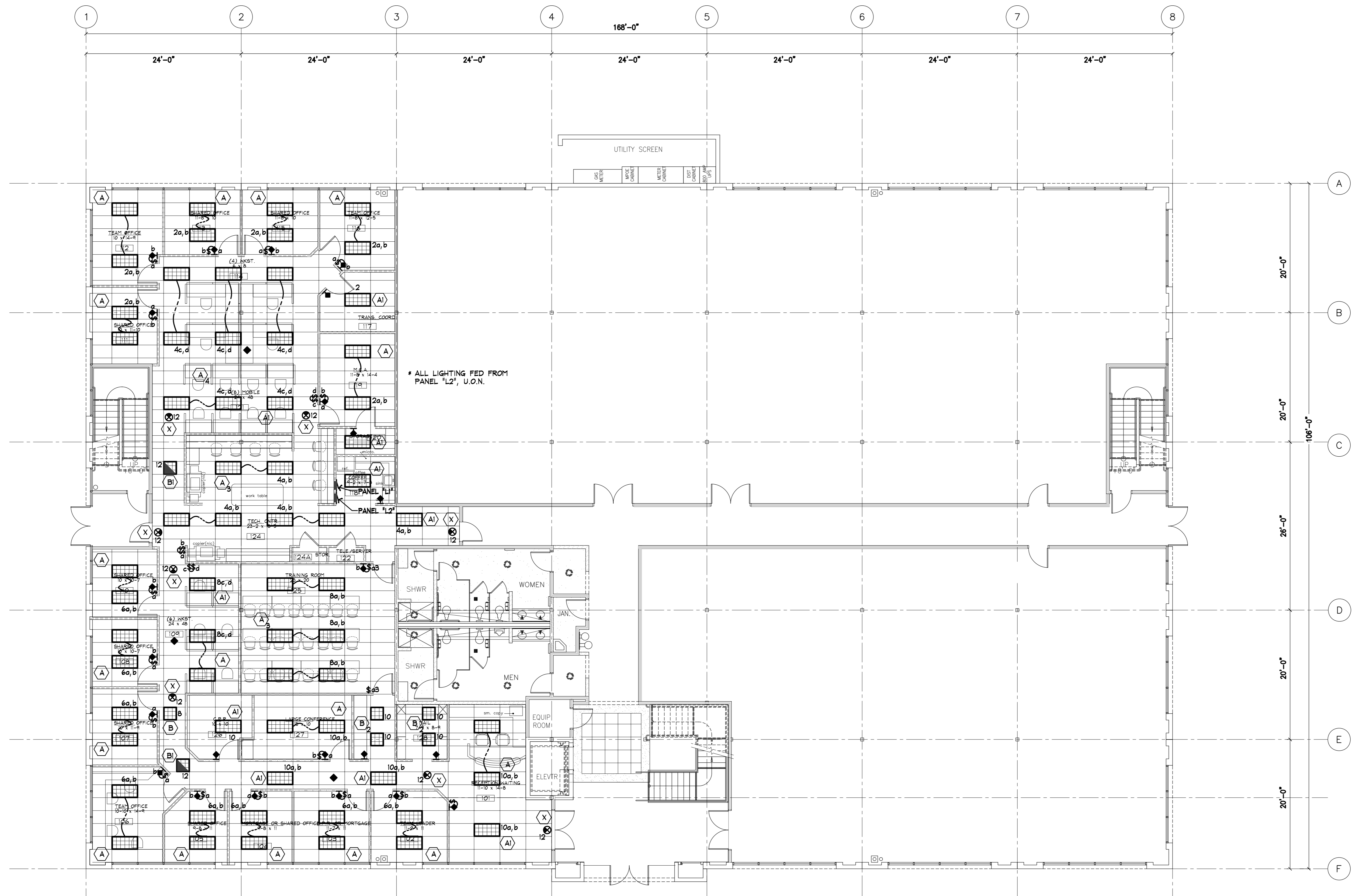
1 1ST FLOOR PLAN (BLDG-2) 1/8" = 1'-0"
