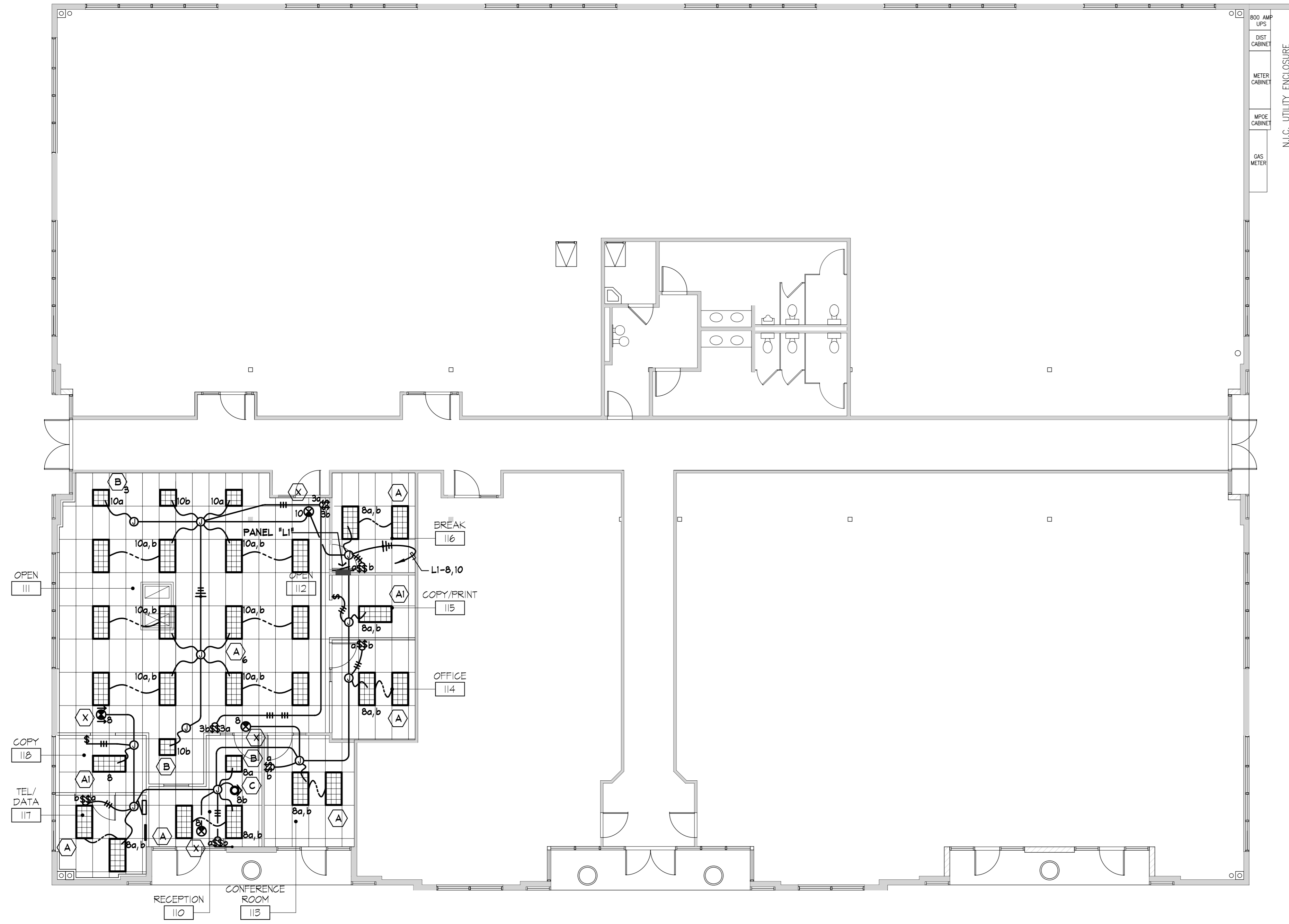
1 FIRST FLOOR LIGHTING PLAN 1/8"=1'-0"
