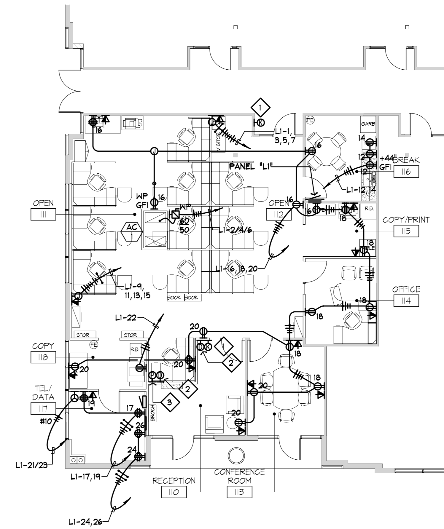
2 FIRST FLOOR POWER PLAN 1/8"=1'-0"
