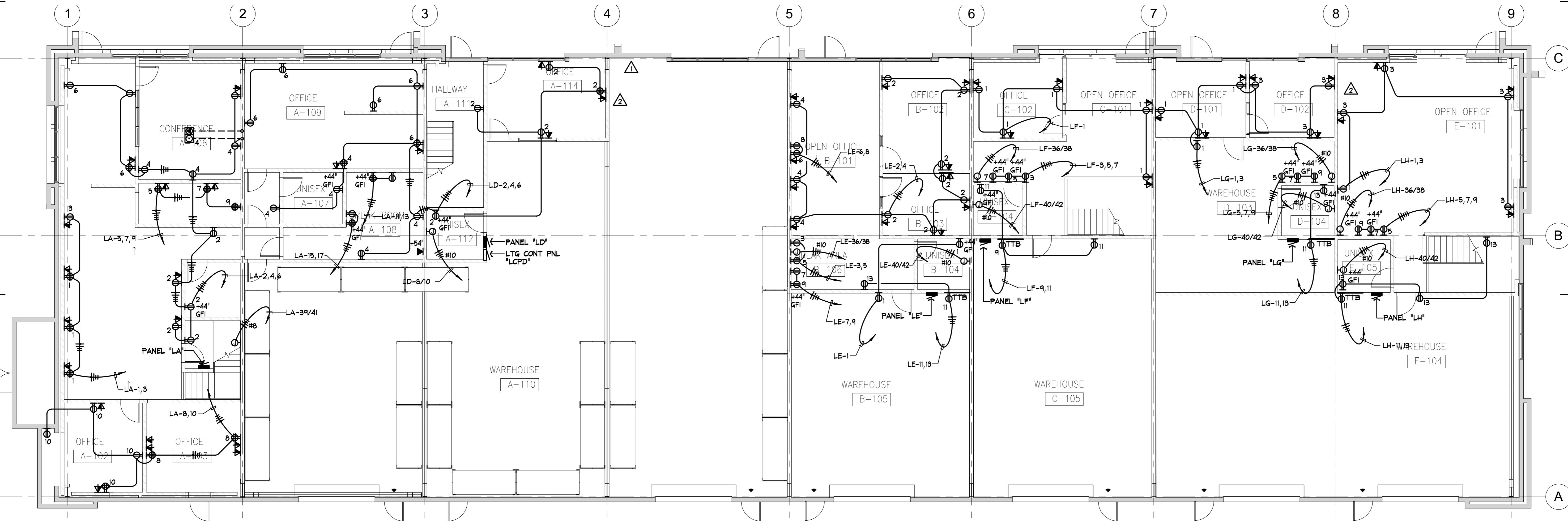
1 FIRST FLOOR POWER PLAN 1/8"=1'-0"
